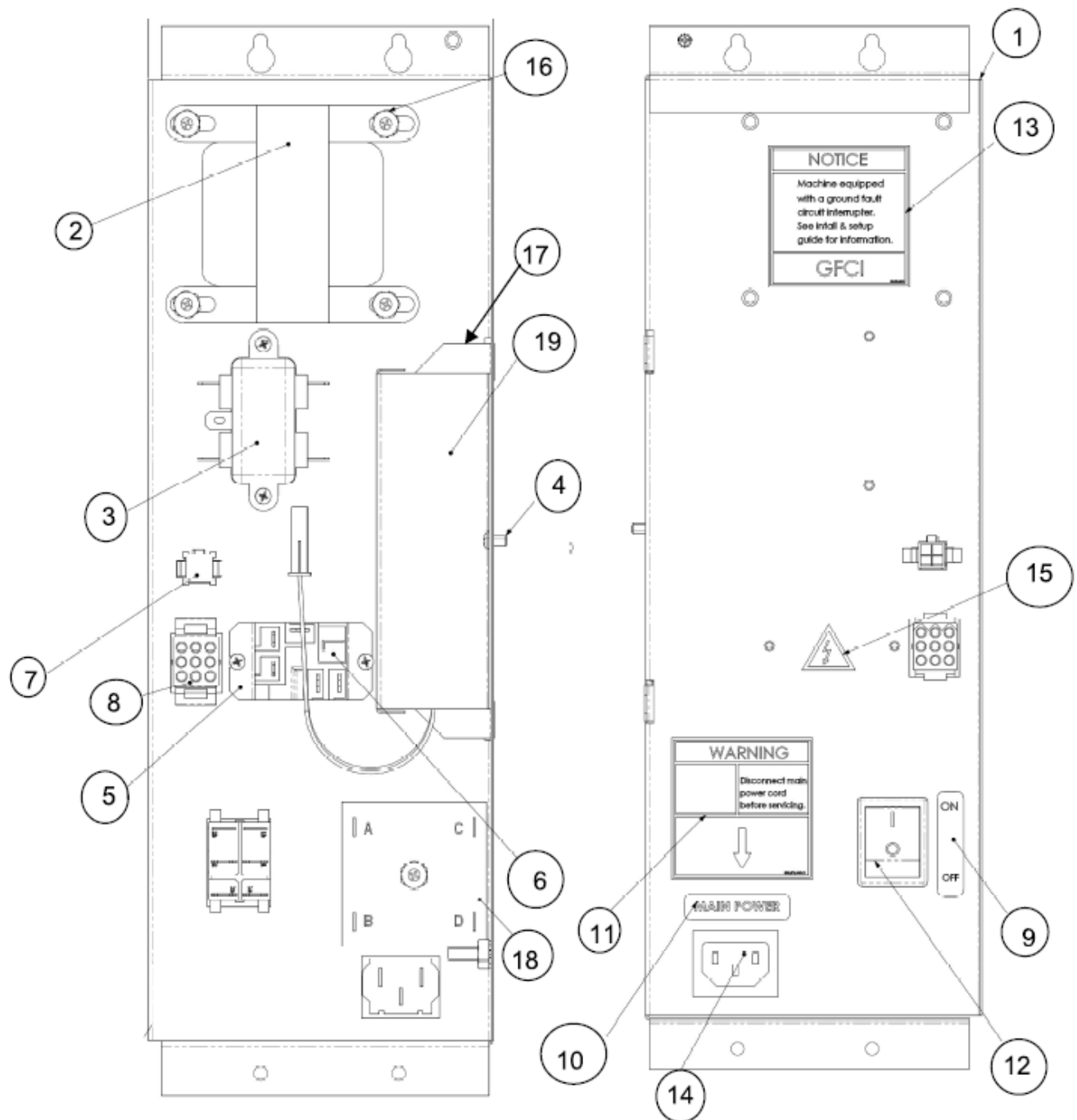
FIGURE 25: ASSY AC BOX – 120VAC
