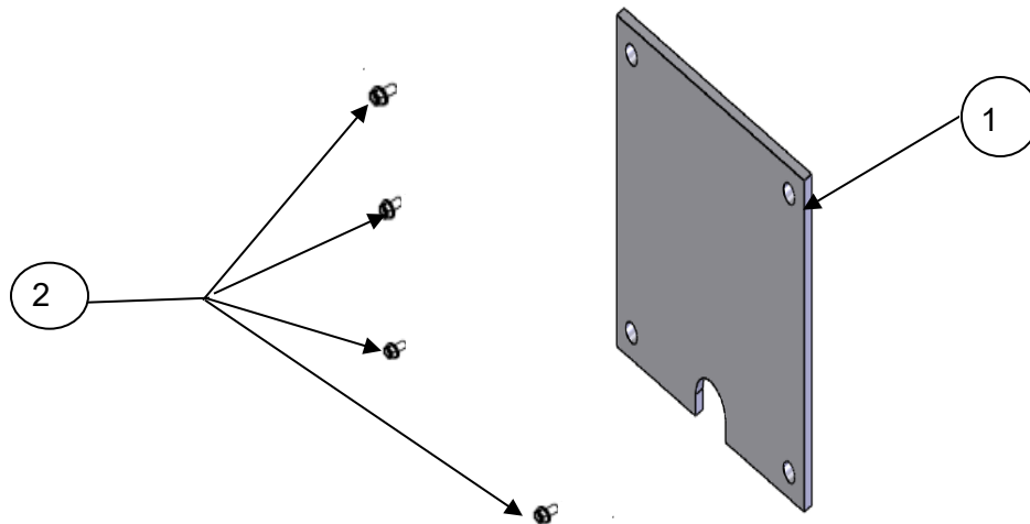
FIGURE 5: COVER, CORD
